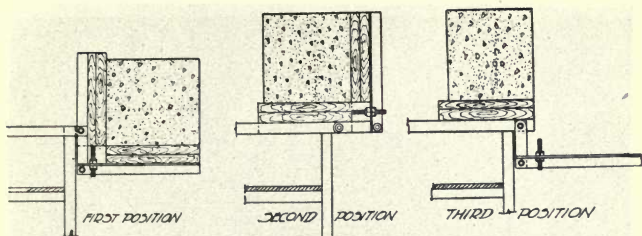
FIG. 73—THREE VIEWS OF TURNING STAND FOR HANDLING GREEN CONCRETE BLOCK TO BE BRUSHED ON THEIR FACE SIDES
